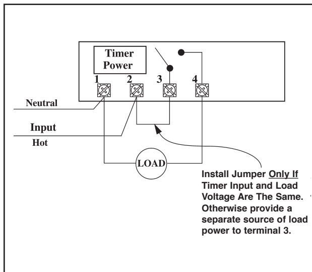
FIG. #4 ET102C SPST
