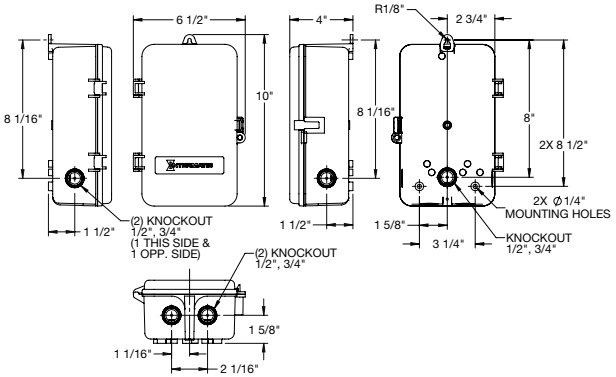
2T2502GA Dimensions
