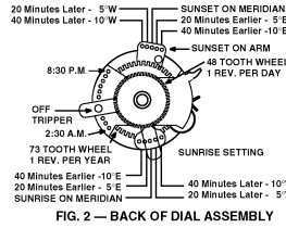
FIG. 2 - BACK OF DIAL ASSEMBLY
