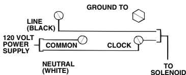
WIRING DIAGRAM
